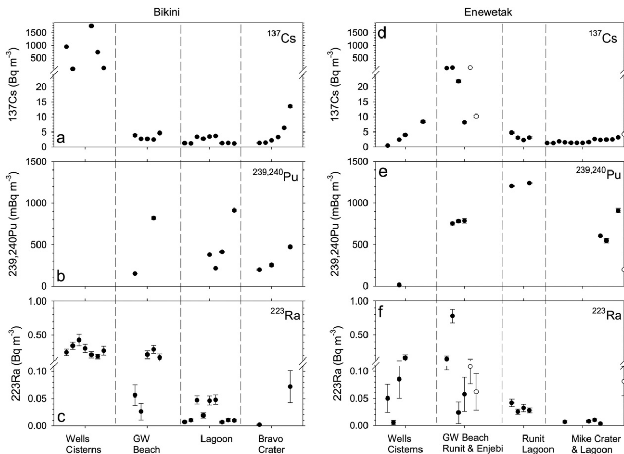
Fig. 3. Comparison of ^{137}\text{Cs} (a, d), ^{239,240}\text{Pu} (b, e) and ^{223}\text{Ra} (c, f) for Bikini (a, b, c) and Enewetak (d, e, f). Data are grouped by type with wells/cisterns on left, followed by the groundwater sampling at the shore line at the beaches (Runit and Enjebi samples distinguished by closed and open symbols, respectively). Lagoon waters are to the right for the average over the Bikini Lagoon, and specific to the Lagoon samples near Runit Dome for Enewetak. The far right set of data in each case is for the Craters at Bravo, and for Enewetak, both crater samples and the lagoon in general. All data are in Table S1 and scales are indicated on the vertical axis.
