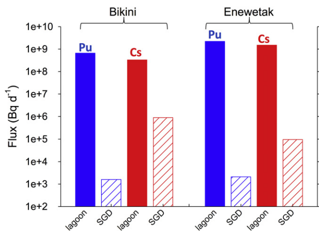
Fig. 7. A comparison of the fluxes ( \text{Bq d}^{-1} ) of ^{239,240}\text{Pu} (blue bars) and ^{137}\text{Cs} (red bars) calculated from the lagoon water exchange rates (solid) and derived from radium based SGD calculations (hatched). The rates for Bikini are on left, Enewetak on right. Details in text and data in Table S3.
