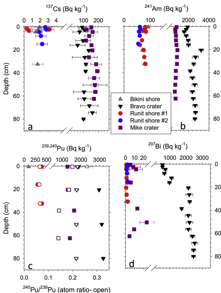
Fig. 5. Sediment core profiles vs. depth (cm- Y axis) for ^{137}\text{Cs} (a), ^{241}\text{Am} (b), ^{239,240}\text{Pu} (c) and ^{207}\text{Bi} (d). For each radionuclide the activities are along the upper x-axis in units of \text{Bq kg}^{-1} dry weight. For Pu, also shown are the ^{240}\text{Pu}/^{239}\text{Pu} atom ratios as open symbols with scale along the lower x-axis. Sample key is shown for Bikini shore (gray triangles), Bravo Crater (black inverted triangles), Runit shore (#1 and #2 are two sites, red and blue circles, respectively) and the Mike Crater (purple square). Error bars are shown if larger than the symbol size for each measurement. Data are in Table S2.
