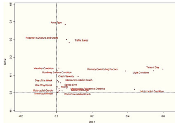
Figure 2. MCA plot of all study variables.
