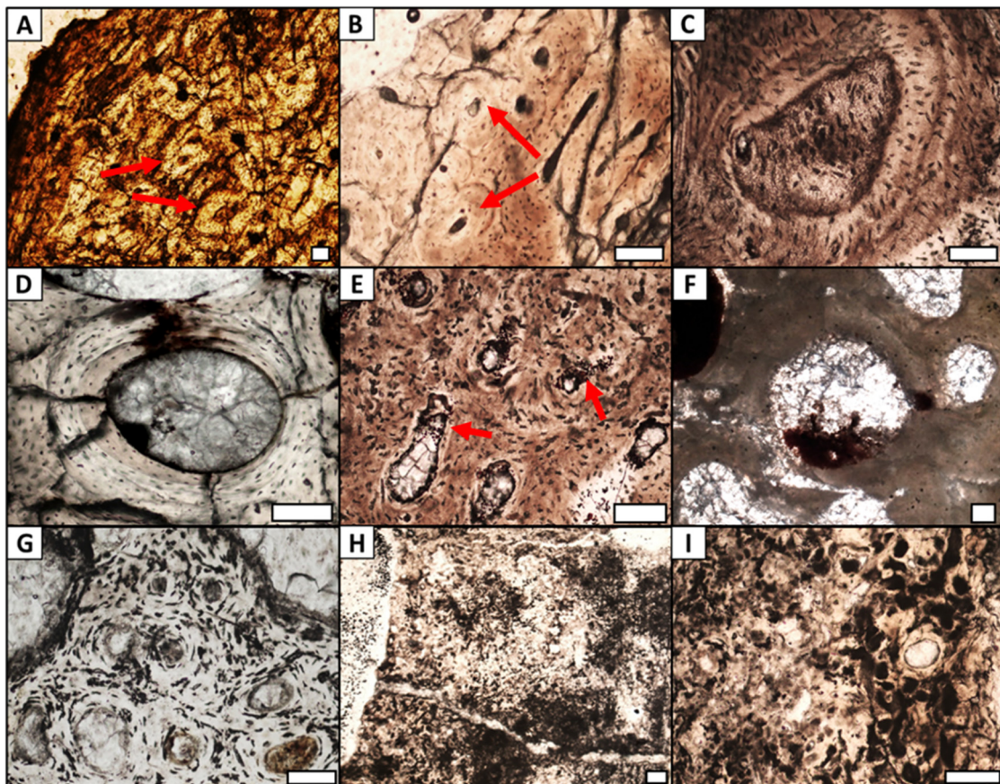
Figure 8. Photomicrographs of thin sections of the White River Group fossil specimens. (A) Haversian systems (red arrows) in the external cortex of a mammal limb bone (Specimen F15). (B) Haversian systems (red arrows) in the external cortex of a mammal rib (FR09-09). (C) Close-up of osteons and osteocytes in the cortical bone of a tortoise shell (F19-06). (D) Sparry calcite
